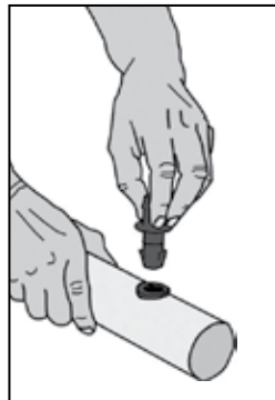
Push XF Series Dripline Insert Adapter into grommet until flange and grommet are flush.
